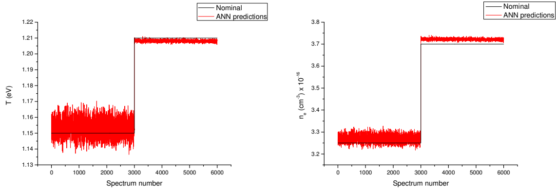
Fig. 11. Predictions of the improved ANN for the spectral parameters of the set of ‘unknown’ LIBS spectra, corresponding to the parameters in Table IV. Left: Electron temperature; Right: Electron number density. The curve in red represents the predictions of the ANN, the one in black the nominal value of the parameters. Each point corresponds to a single LIBS spectrum.
