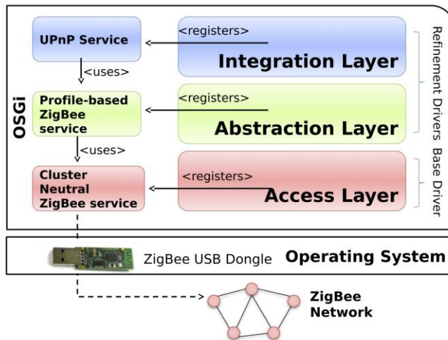
Figure 1: The ZB4O architecture.
