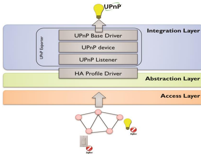
Figure 2: The UPnP Exporter.
