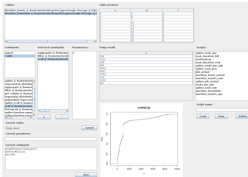
Fig. 2: Screenshot of the BiDAL analysis console displaying R commands.
