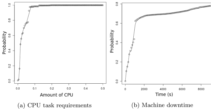
Fig. 5: Examples of CDFs fitted by sequences of splines, obtained with BiDAL. The circles represent the data, while the lines show the fitted splines.
