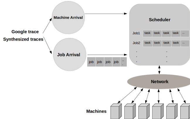
Fig. 6: Architecture of simulation model.
