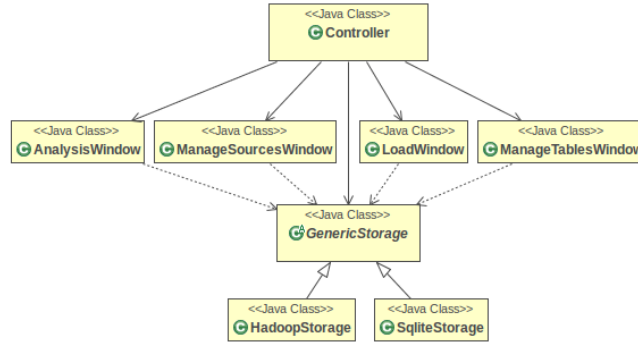
Fig. 1: UML diagram of BiDAI classes.
