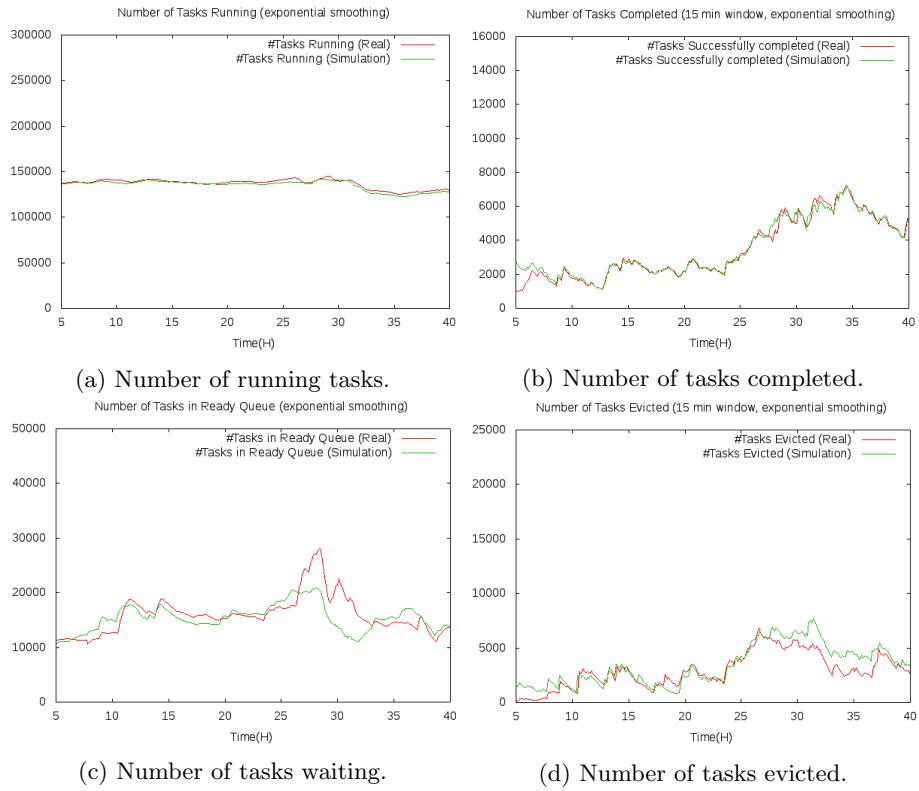
Fig. 7: Simulation and real data for four different metrics.
