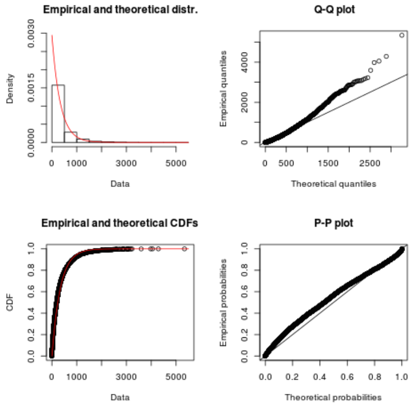
Fig. 4: Machine update events, fitted with an exponential distribution. The left panels show the density and cumulative distribution functions, with the lines representing the exponential fitting and the bars/circles showing real data. The right panels show goodness of fit in Q-Q and P-P plots (straight lines show perfect fit).
