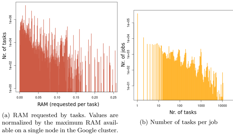
Fig. 3: Examples of distributions obtained with BiDAL.
