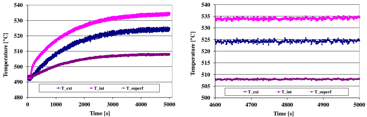
Figure 4. Hot wire test results at 500°C.
