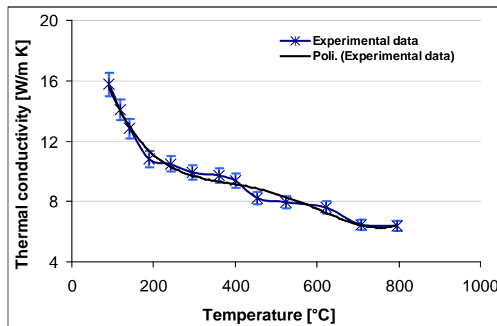
Figure 5. Thermal conductivity vs. temperature.
