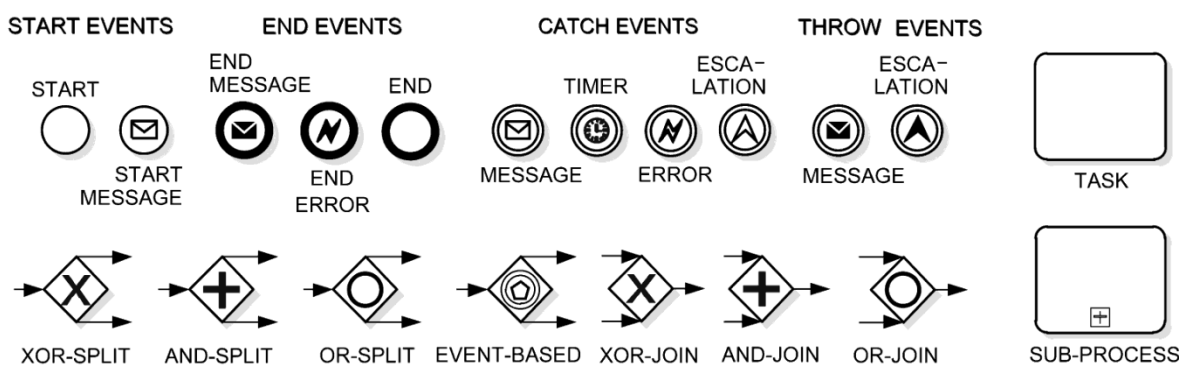
Figure 1. Business Process Model and Notation (BPMN) elements supported by the Bimp simulator.
