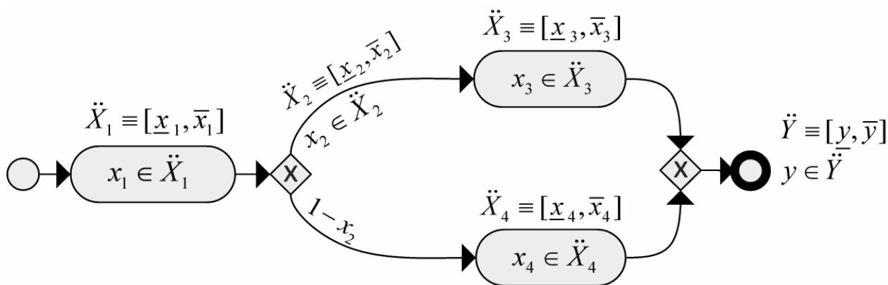
Figure 6. A simple case of interval-valued BPMN model.
