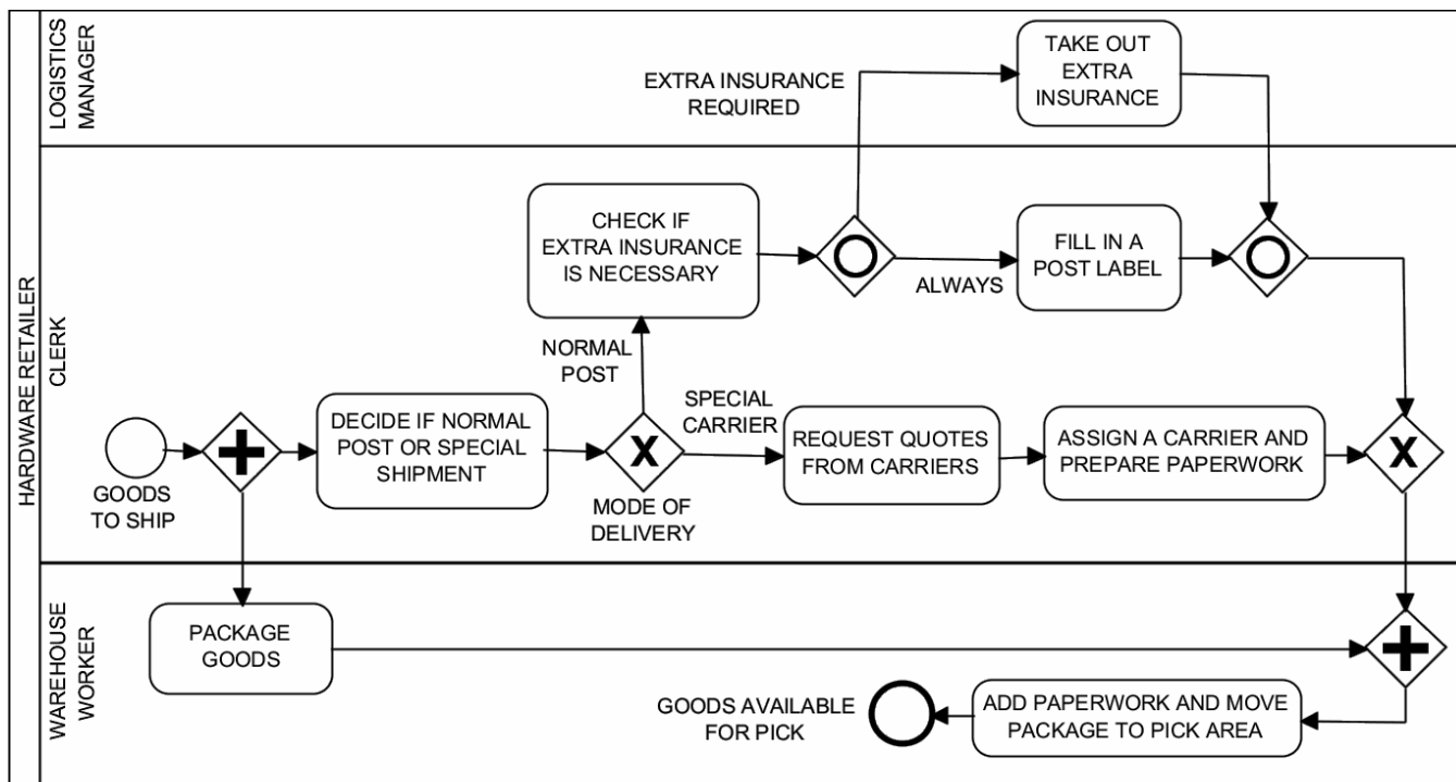
Figure 12. Shipment process of a hardware retailer: BPMN process diagram.
