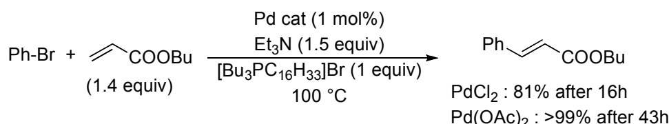
Scheme 1. Heck reaction without additive ligands in [C 16 PBu 3 ]Br.
