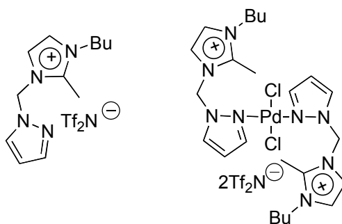
Figure 1. Palladium complex from N-pyrazolyl 2-methyl imidazolium based IL.
