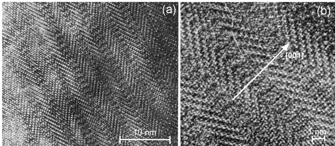
Fig. 1. HRTEM image of sacrofanite, zone axis [100].
