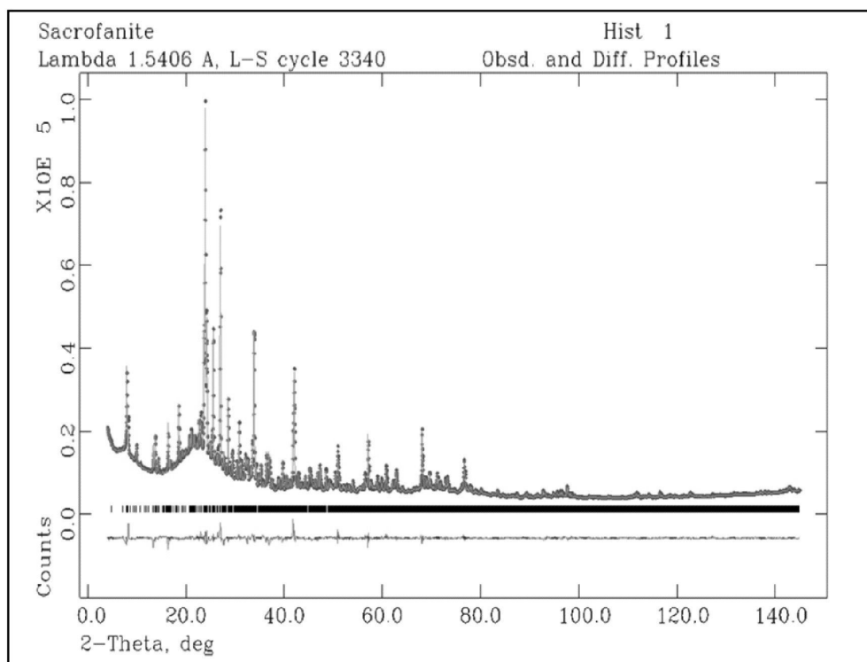
Fig. 2. Experimental (dots) and calculated (continuous line) Rietveld plots for sacrofanite. The difference profile is shown at the bottom of the figure. Vertical markers refer to the position of the calculated Bragg reflections.
