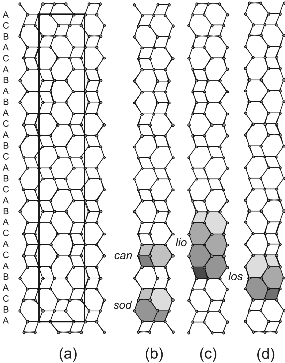
Fig. 3. Schematic drawing of the framework of sacrofanite, projected along [100]. In (a) the unit cell is outlined. For sake of simplicity, the cages that are superimposed along [0, 0, z] , [1/3, 2/3, z] , and [2/3, 1/3, z] , are shown separately in (b), (c) and (d), respectively. lio = liottite cage [4^66^{17}] ; los = losod cage [4^66^{11}] ; sod = sodalite cage [4^66^8] ; can = cancrinite cage [4^66^5] .
