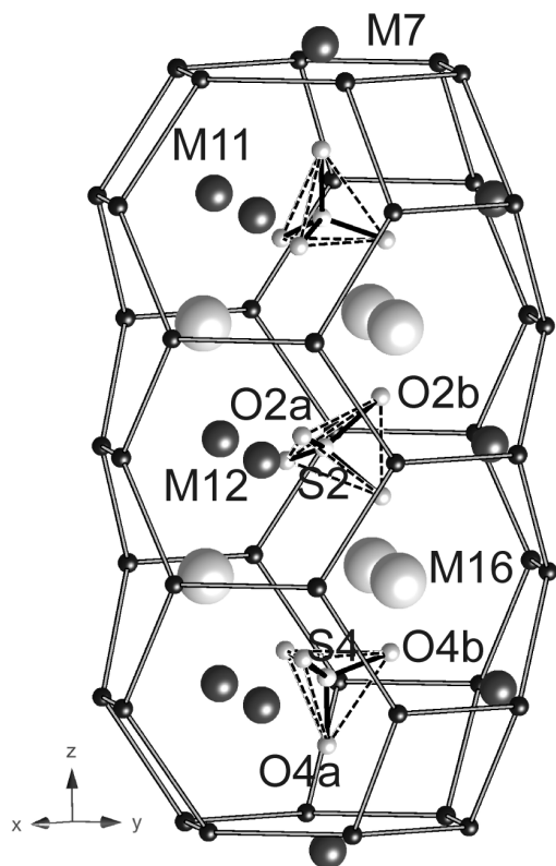
Fig. 4. Liottite cage in sacrofanite. The S2-centred tetrahedron, with S2 placed on the mirror plane at z = \frac{1}{4} , may statistically assume different orientations. For sake of clarity, only one of them is shown.
