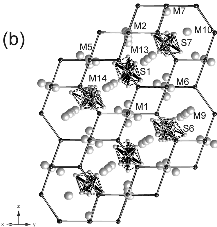
Fig. 7. Cancrinite cages in sacrofanite. In (a) the two symmetry-independent cancrinite cages located along the six-fold axis are shown. The F1 and F3 sites host fluorine
