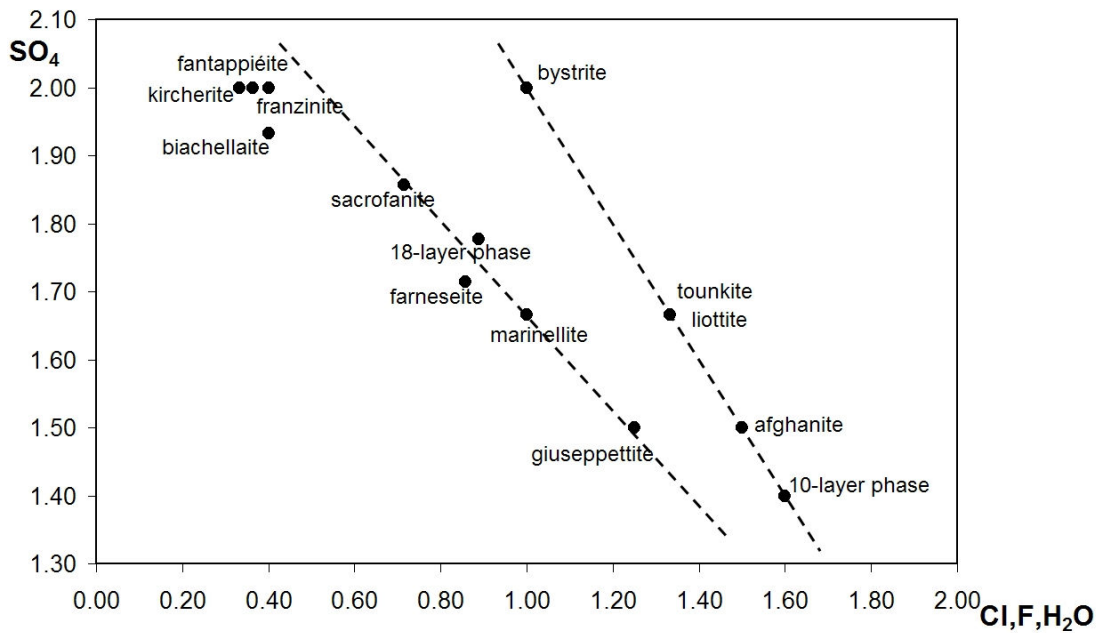
Fig. 8. Different compositional fields of the phases with a complex sequences of layers.
