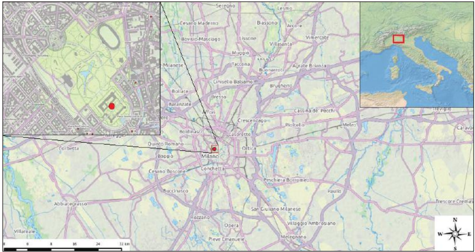
Figure 6. Distribution map of Hieracium australe subsp. australe .
