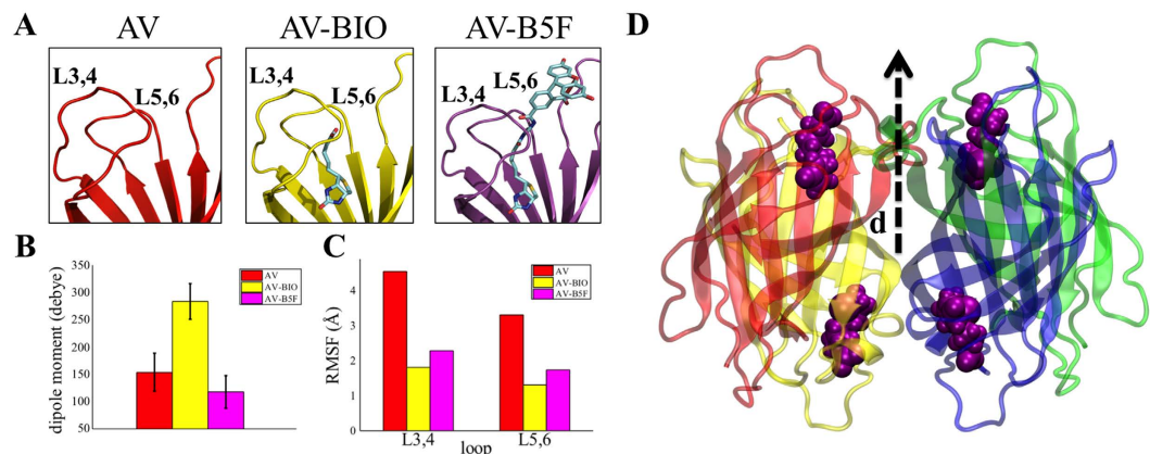
Figure 4. Molecular dynamics simulations of Biotin-binding proteins. (A) Residues close to the binding pocket of the AV (left), AV-Biotin complex (center) and Avidin-B5F complex (right). (B) Histogram showing the dipole moment (Debye) averaged along the obtained molecular dynamics trajectory for AV (red), AV-Biotin (yellow) and AV-B4F (magenta) systems. A single value is reported for each system averaging statistics from the two monomers. (C) Histogram showing the computed Root Mean Square Fluctuations (RMSF) (Å) values for AV (red), AV-BIO (yellow) and AV-B4F (magenta) systems considering both L3,4 and L5,6 loops. For each system, the averaged RMSE, computed from the two monomers, is reported. (D) Overall tetrameric structure of the simulated AV with bound biotin molecules. Dipole directions are shown (not to scale).
