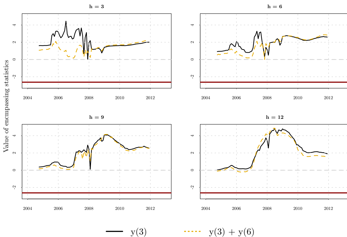
Figure 3. Testing the condition in Proposition 1
