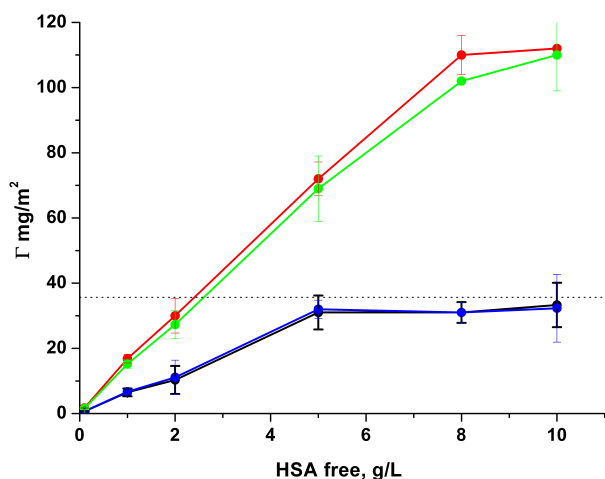
Figure 5. HSA amounts, surface interacting with the different TiO 2 nanocrystals: TA (black); TO (green); TB (blue); P25 (red). Data were expressed as HSA amount adsorbed per square metre versus the free protein concentration in the supernatant, after 1 h of incubation. The dotted horizontal line indicates the HSA adsorbed amount needed to build up a theoretical monolayer on a flat surface.
