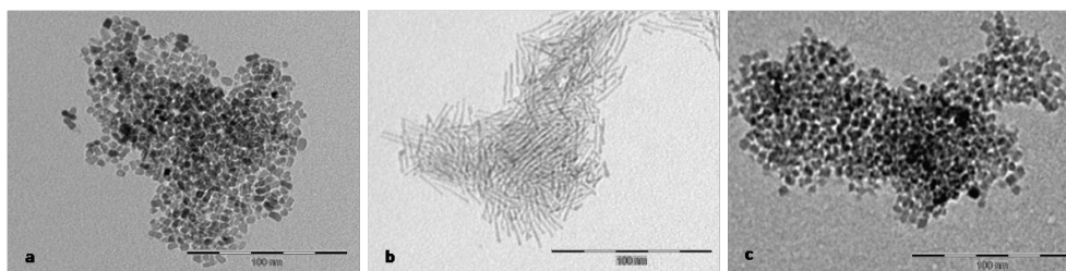
Figure 1. TEM images of the different TiO 2 samples: (a) TA, (b) TO, (c) TB
