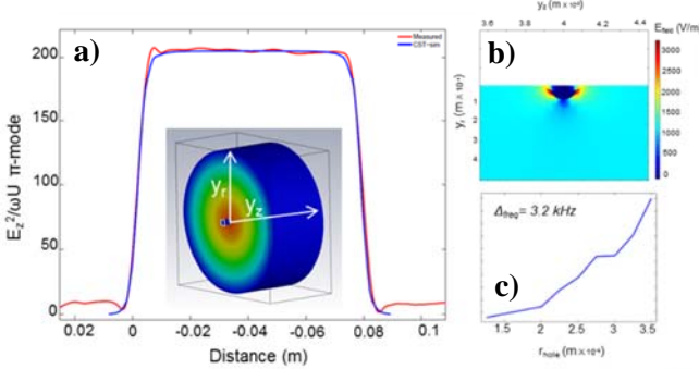
Figure 2: Comparison field profile extracted from EM simulations and pill-box measurements (a). Field profile simulation for a hollowed bead (b). Frequency shift induced for different bead holes radii (c).
