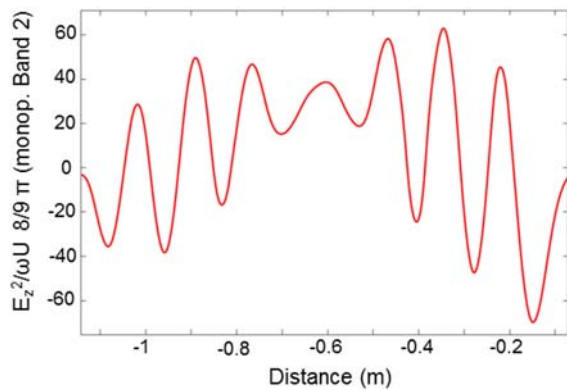
Figure 4: Measured HOM E_z^2/\omega U profile for the 8/9\pi -mode in the second monopole band, f(8/9\pi)=2.45\text{GHz} .
