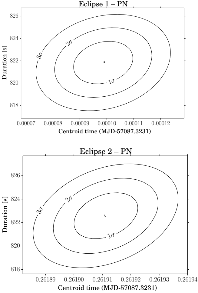
Fig. 6. Contour plots of the two eclipses durations and mid-pochs obtained by fitting the rectangular eclipse model to the data. The 1\sigma , 2\sigma , and 3\sigma contours around the best determined values are indicated.
