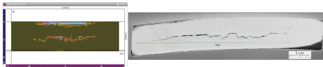
Fig. 5. HIC detected with FMC/TFM. Sample B
