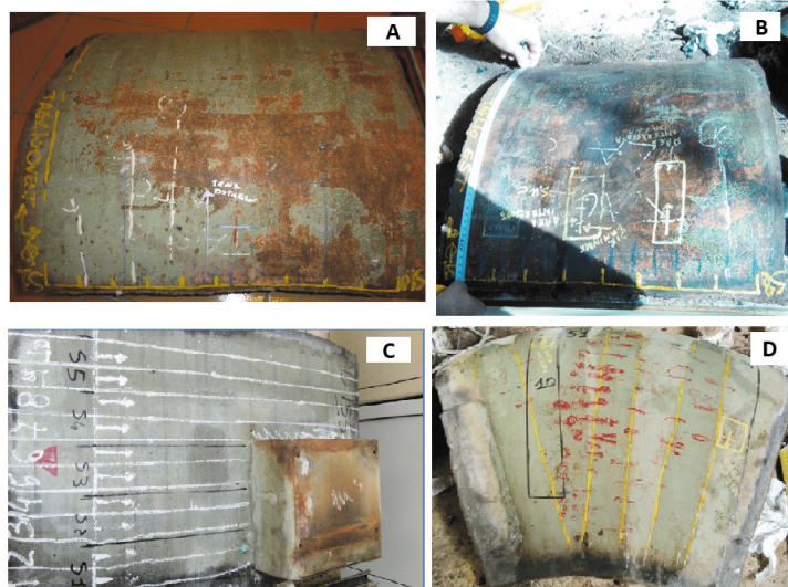
Fig. 1. Test pieces
