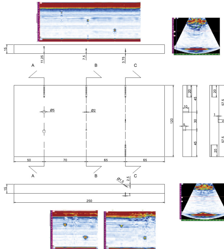
Fig. 2. Calibration block design and related PA scan
