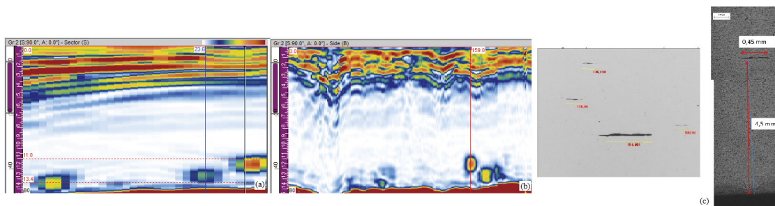
Fig. 6. Planar inclusions (nonmetallic). E-Scan (a) and B-scan (b) vs macro (c). Sample D
