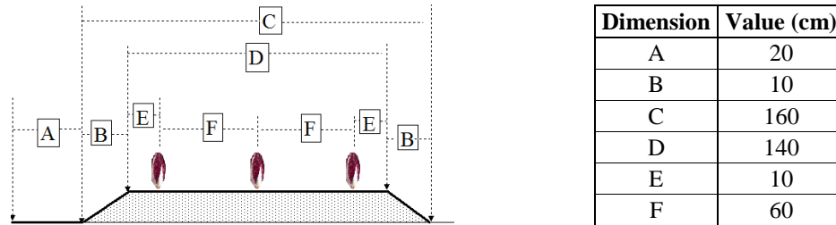
Figure 2 – Schematic of the seed-bed prepared with the “TSA 190” machine (the seed-bed height is not indicated, as it was object of the study presented here).
