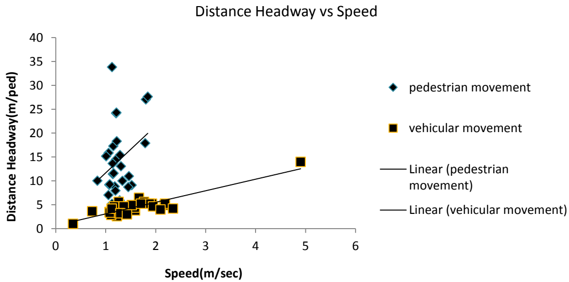
Figure: 4.3.1 (b) Distance headway – speed plot for Bisra Chowk and Ambagan, Rourkela.
