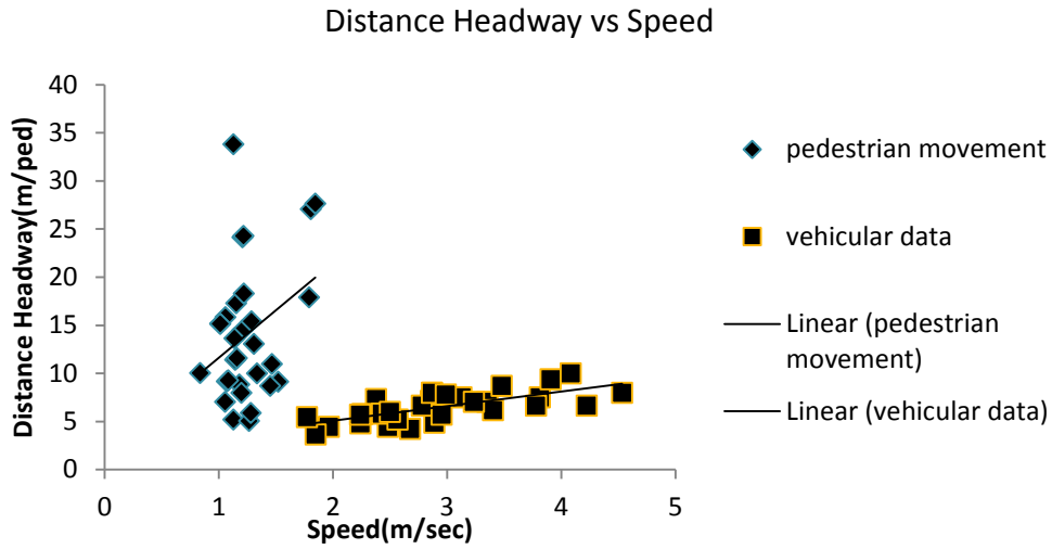
Figure: 4.3.1 (a) Distance headway – speed plot for Ambagan and Ambagan, Rourkela.
