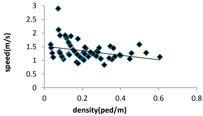
Figure: 4.2.1 Speed density plot for (a) Ambagan, Rourkela
