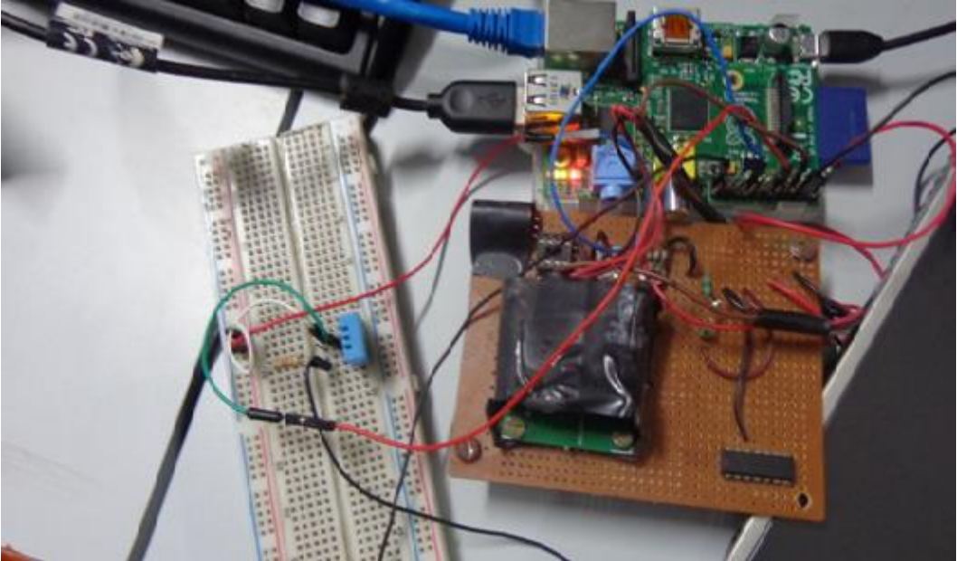
Figure 3-15 Hardware set up for temperature sensing, pulse rate and the video conferencing.
