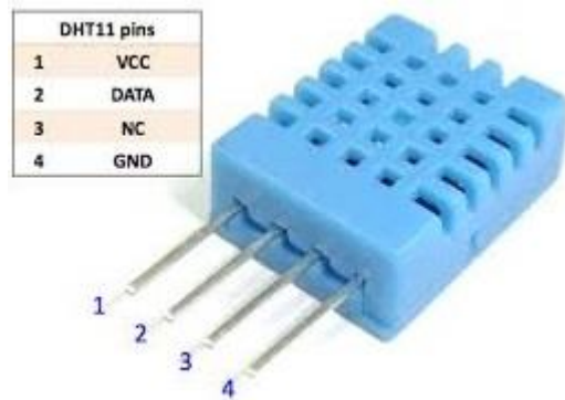
Figure 3- 4 DHT11 sensor
