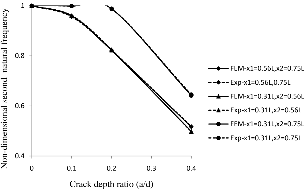
Figure 5.19 Comparison of FEM and experimental results for non-dimensional second natural frequencies of double cracked free-free beam with crack depth ratio (a/d) for different locations of crack.
