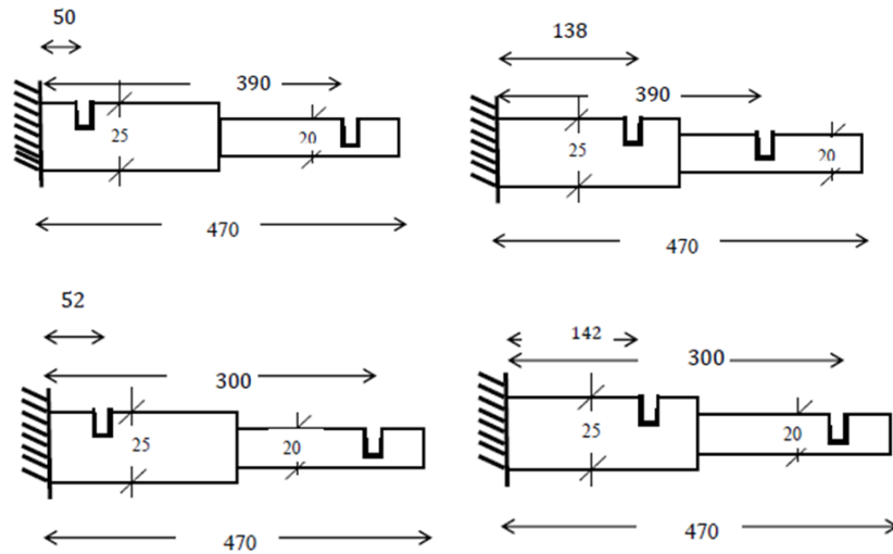
Figure 5.41 Sketch of stepped fixed-free beam with two cracks considered at different locations for the present study.
