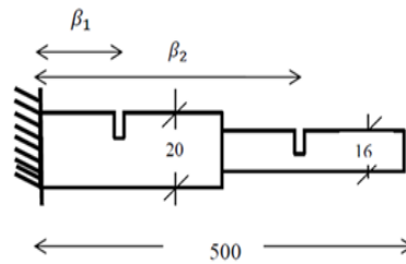
Figure 5.4 Cracked cantilever stepped beam (mm)
