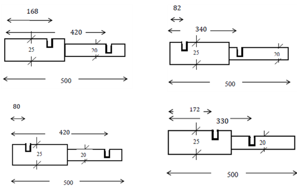
Figure 5.37 Sketch of stepped free-free beam with two cracks considered at different locations for the present study.
