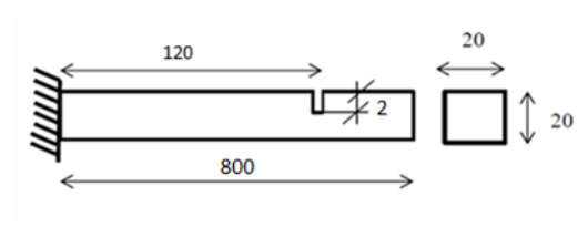
Figure 5.3 Cracked cantilever beam (mm)
