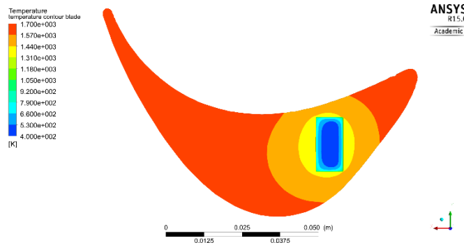
Figure 4.1-3: Temperature contour of the blade body for m = 0.02 \text{ kg/s}
