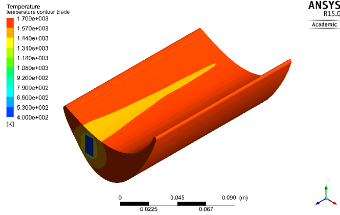
Figure 4.1-2: Temperature contour of the blade body for m = 0.01 \text{ kg/s}
