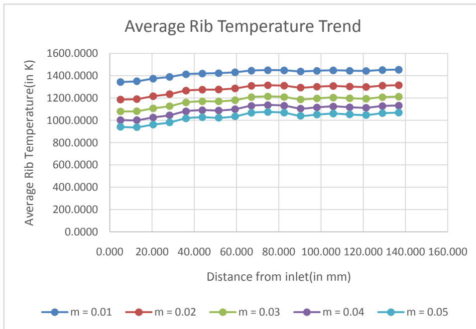
Figure 4.3-1: Variation of average rib temperature, for various mass flow rates
