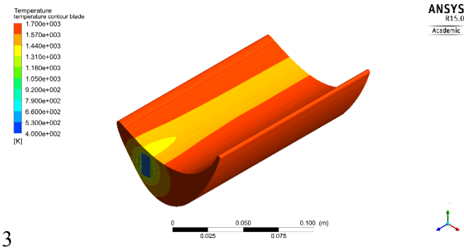
Figure 4.1-3: Temperature contour of the blade body for m = 0.02 \text{ kg/s}
