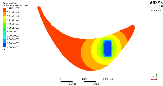
Figure 4.1-10: Temperature contour at outlet of the passage for m = 0.05 \text{ kg/s}
