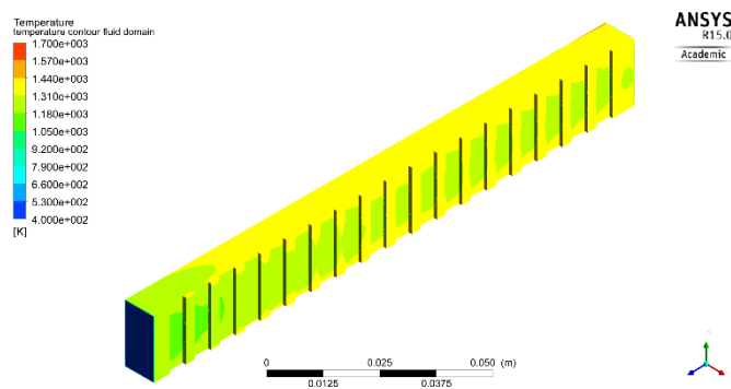
Figure 4.2-3: Temperature contour of the fluid domain for m = 0.03 kg/s
