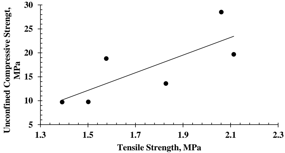
Figure 5.2:- Relation between UCS and Tensile Strength (Linear)
