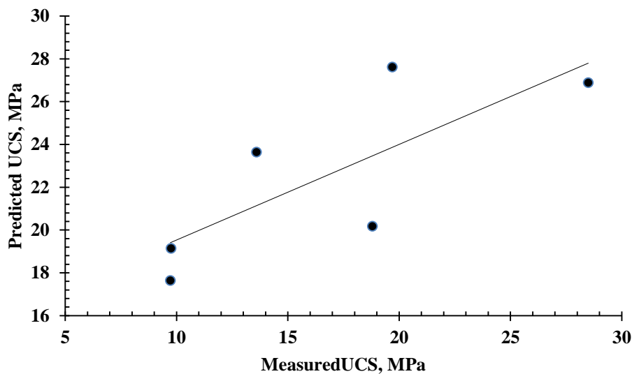
Figure 5.17:- Measured UCS vs. Predicted UCS by Altindag and Guney
