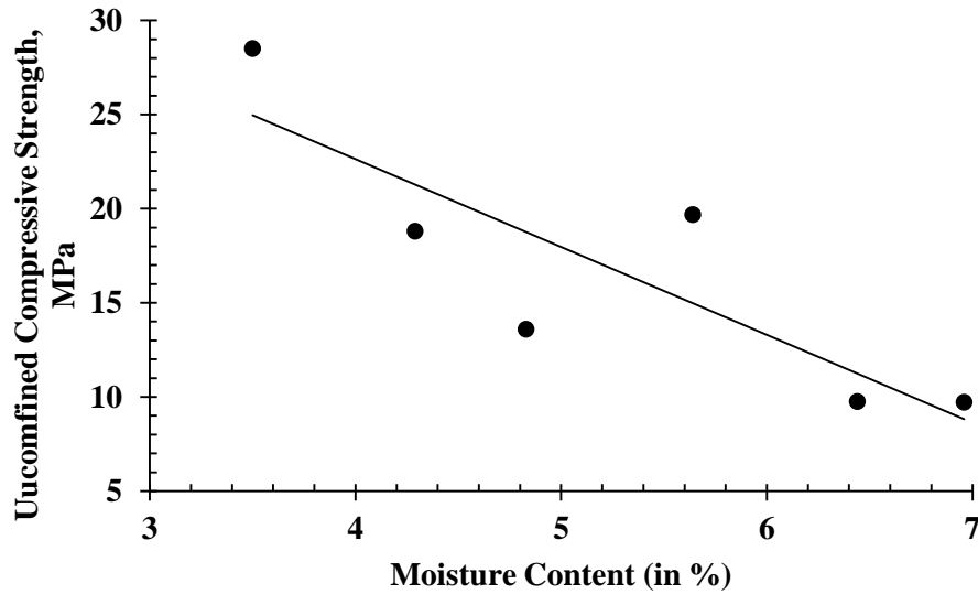
Figure 5.4:- Relation between UCS and Moisture Content
