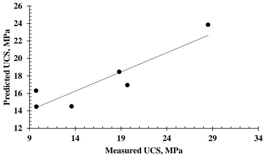
Figure 5.10:- Measured UCS vs. Predicted UCS by Broch and Franklin
