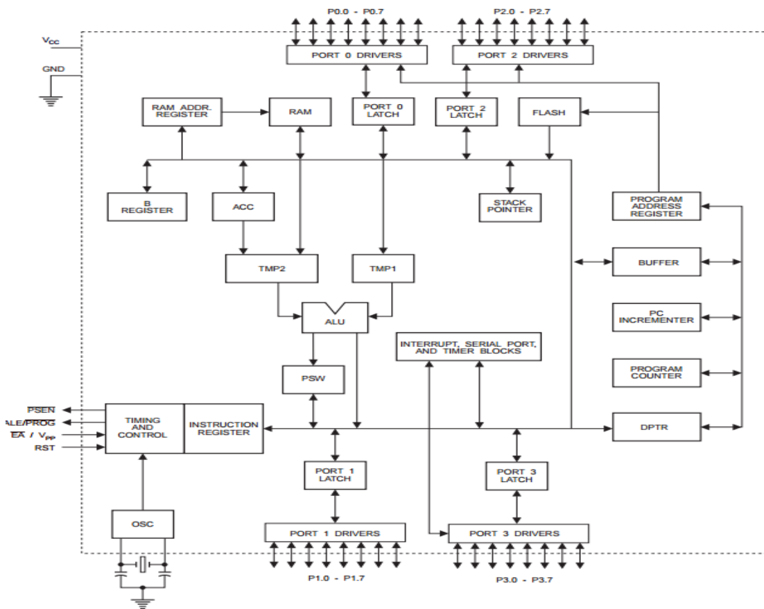
Fig. 19 – 8051 internal schematics.
