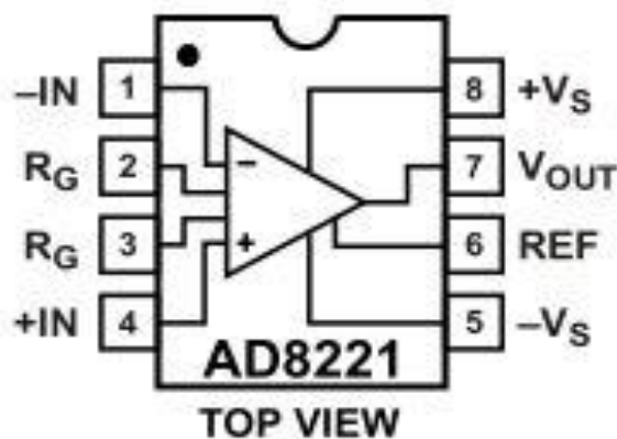
Fig. 8 – Connection diagram
