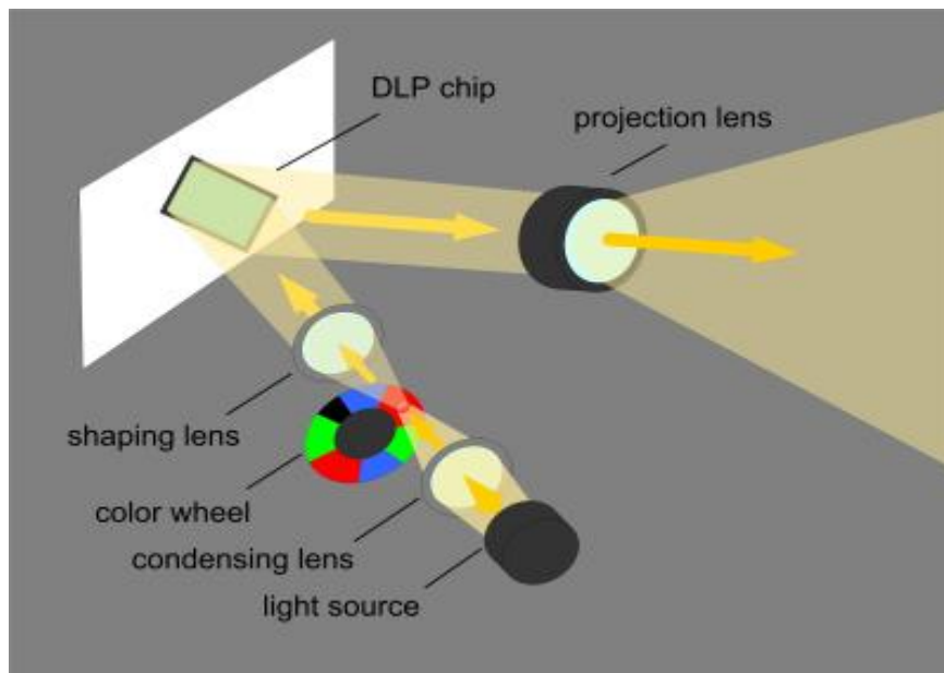
Fig- 13: Illustration of DLP Projection
