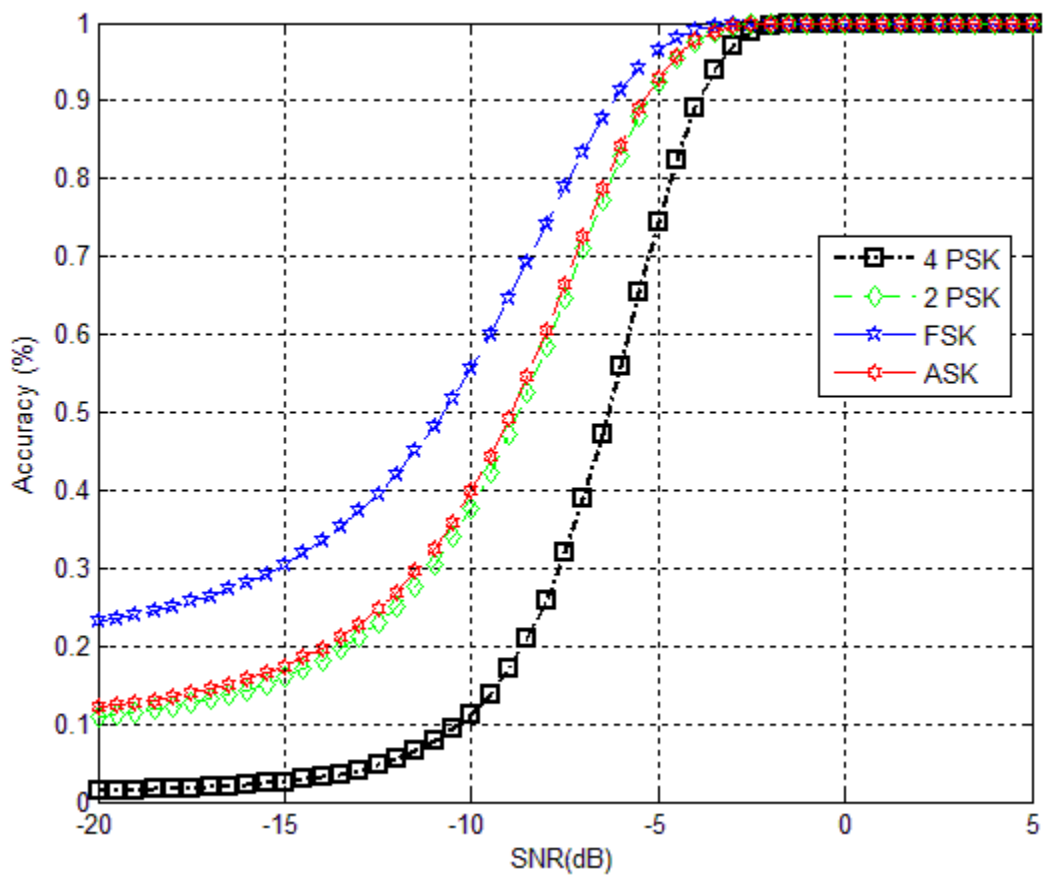
Figure 4.3: Accuracy Vs SNR plot for digital signal
