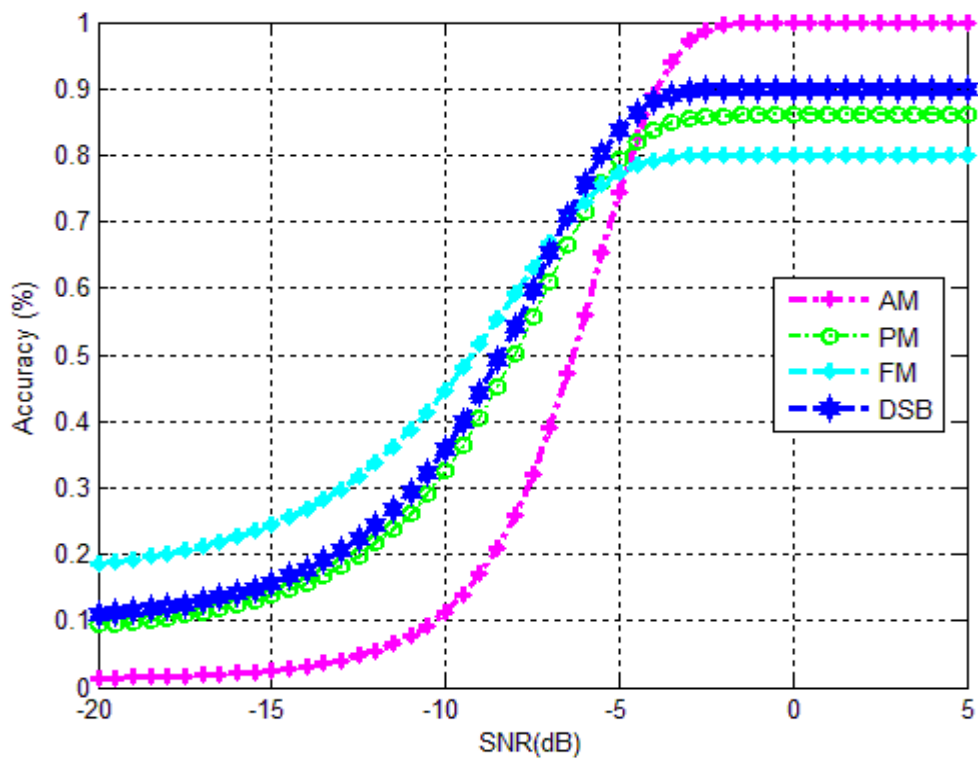
Figure 4.2: Accuracy vs. SNR plot for analog signal
