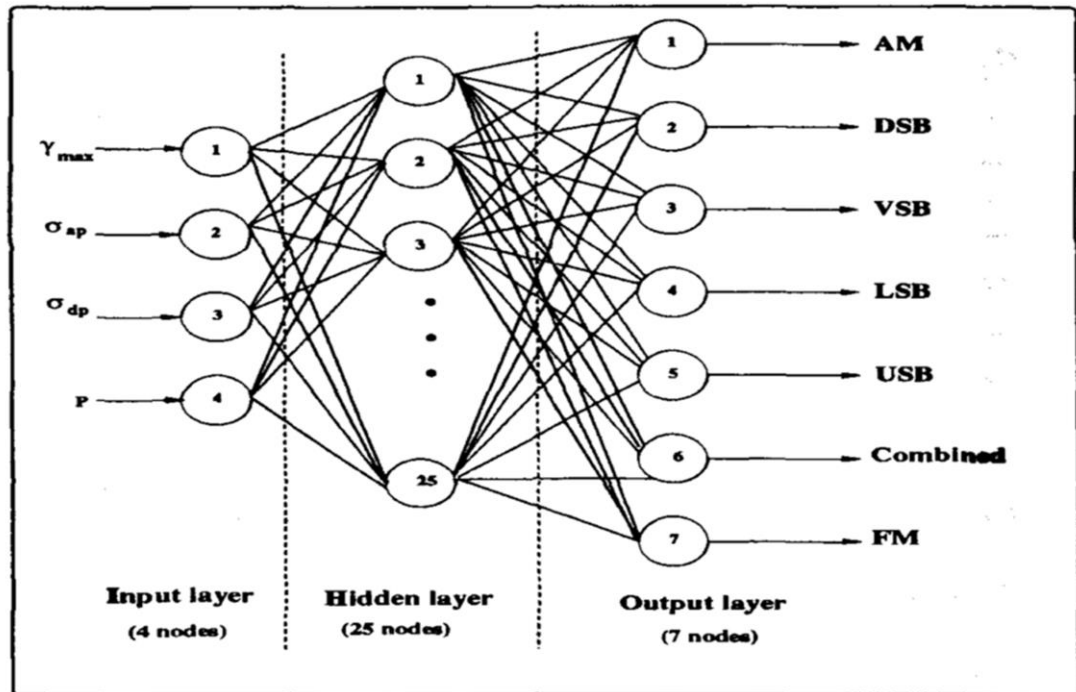
Figure 3.10 Neural networks with one hidden layer, four input node and seven output node
