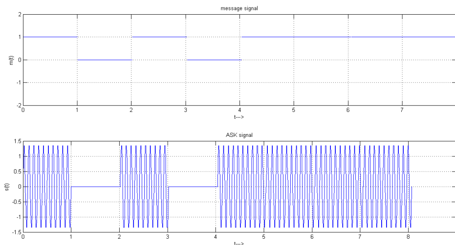
Figure 3.7: ASK modulated signal
