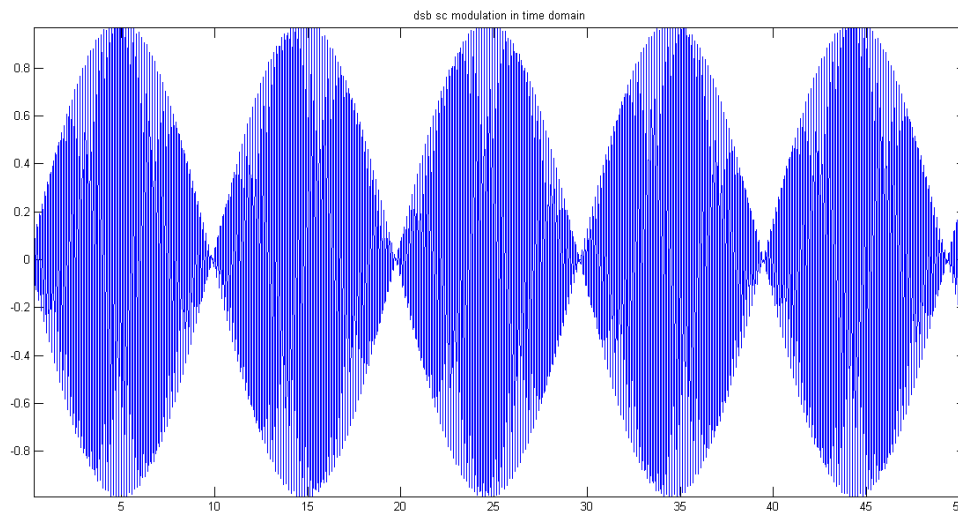
Figure 3.3: DSB-SC modulated signal
