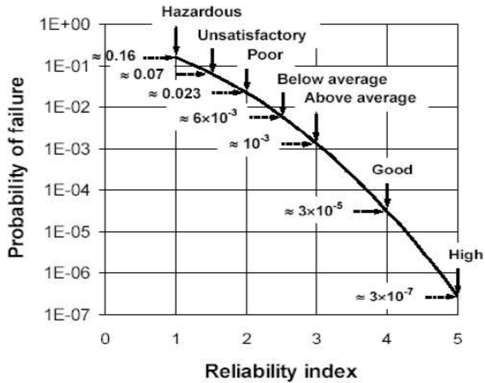
Fig 2.8: Chart between the Reliability index ( \beta ) and the probability of failure ( P_f ) (USACE 1997)
