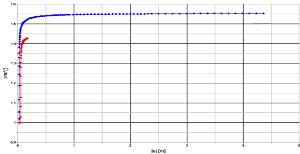
Fig 5.3: Total displacement (U) Vs Incremental multipliers ( M_{sf} )
