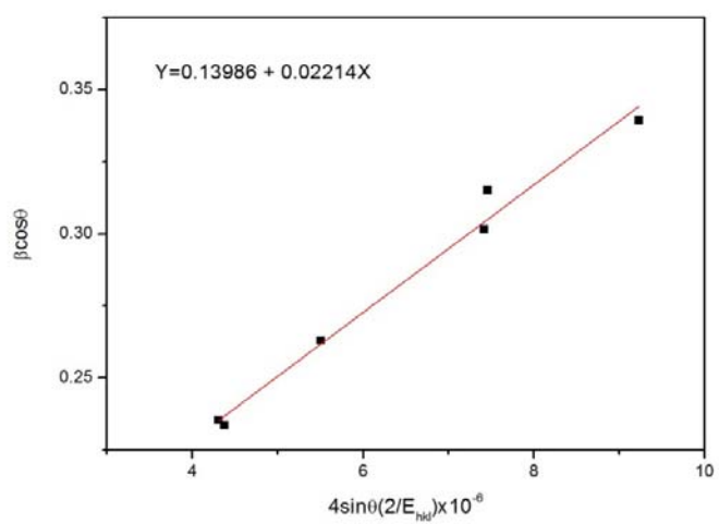
Figure 8: Different plots of zinc oxide powders, calcined at 600 °C.
