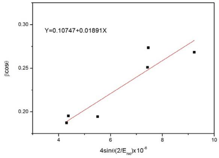
Figure 9: Different plots of zinc oxide powders, calcined at 800 °C.
