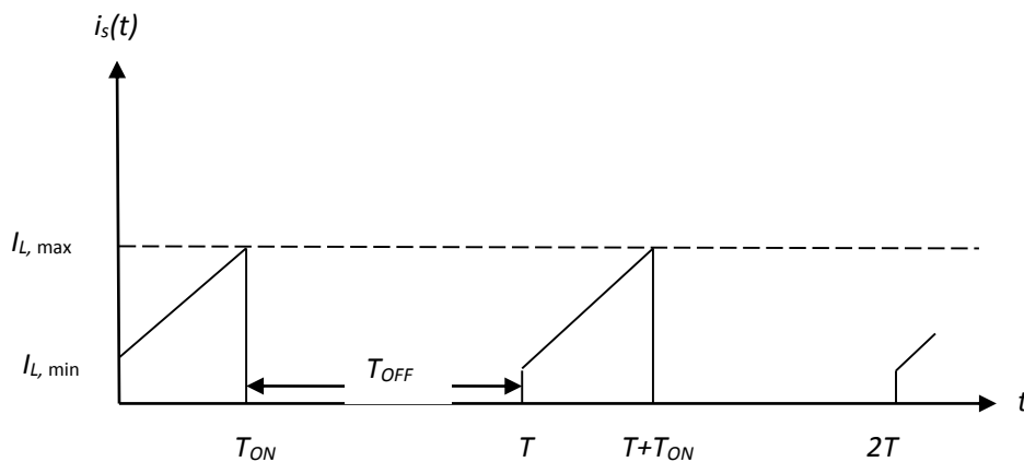
FIGURE 15.2: THE SOURCE CURRENT
