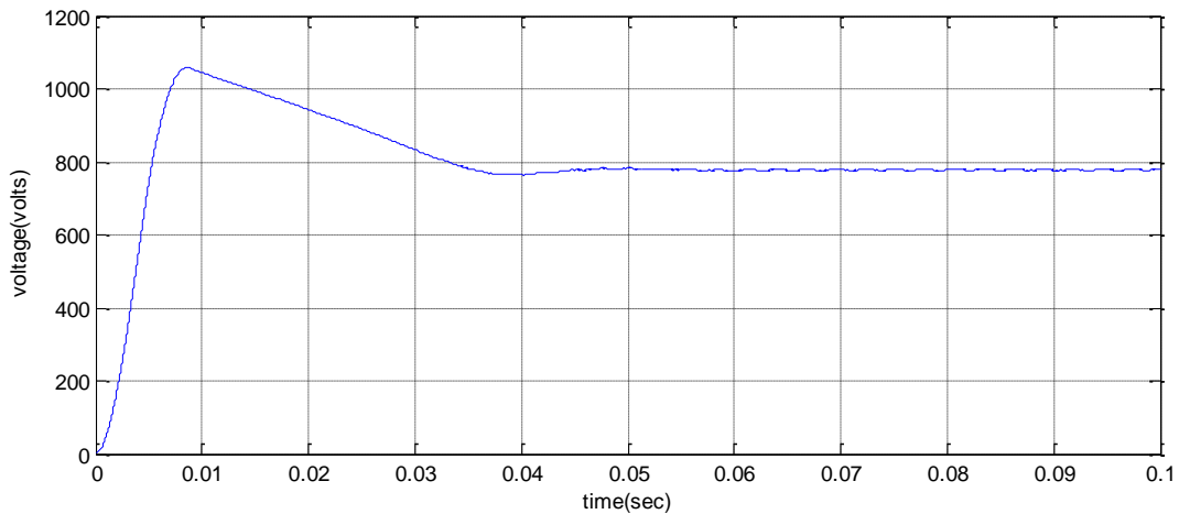
FIGURE 21: GRAPH OF V DC (VOLT) VS TIME (SEC)
