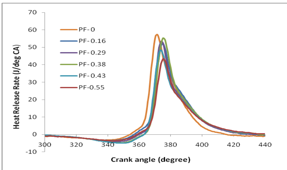
Fig. 4.6 Variation of heat release rate with crank angle at low load
