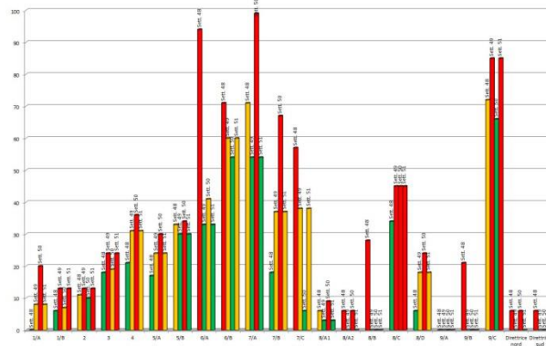
Fig. 3 Overcrowding histograms.
