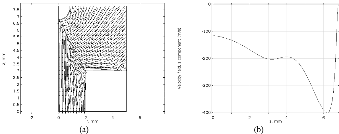
Figure 3. Plasma velocity fields: a) – streamlines of plasma fluxes; b) – velocity of arc plasma on the axis.
