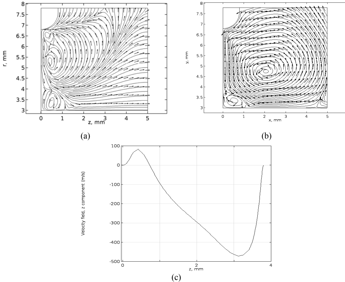
Figure 2. Velocity field of arc: (a) - streamlines at t=1.1 \mu\text{s} ; (b) - streamlines at t=8 \text{ ms} ; (c) - v_z on the axis of symmetry GE ( t=8 \text{ ms} )
