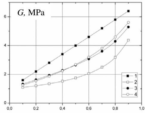
Figure 2. Effective characteristics dependi \gamma_1 on \gamma_1 . 1, 2 –modules Voigt and Reuss, 3, 4 – G_{S,VR}, G_{S,HS} .
