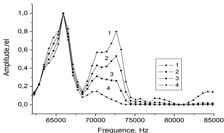
Figure 3. Power spectrum of the electromagnetic response at the excitation pulse frequency of 65 kHz with different pulse duration: 1 – 12 \mu s, 2 – 33 \mu s, 3 – 66 \mu s and 4 – 100 \mu s.
