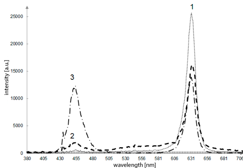
Figure 2. Radiation spectra of experimental LED modules. 1) is PhT No. 1, 2) is PhT No. 3 and 3) is PhT No. 3.
