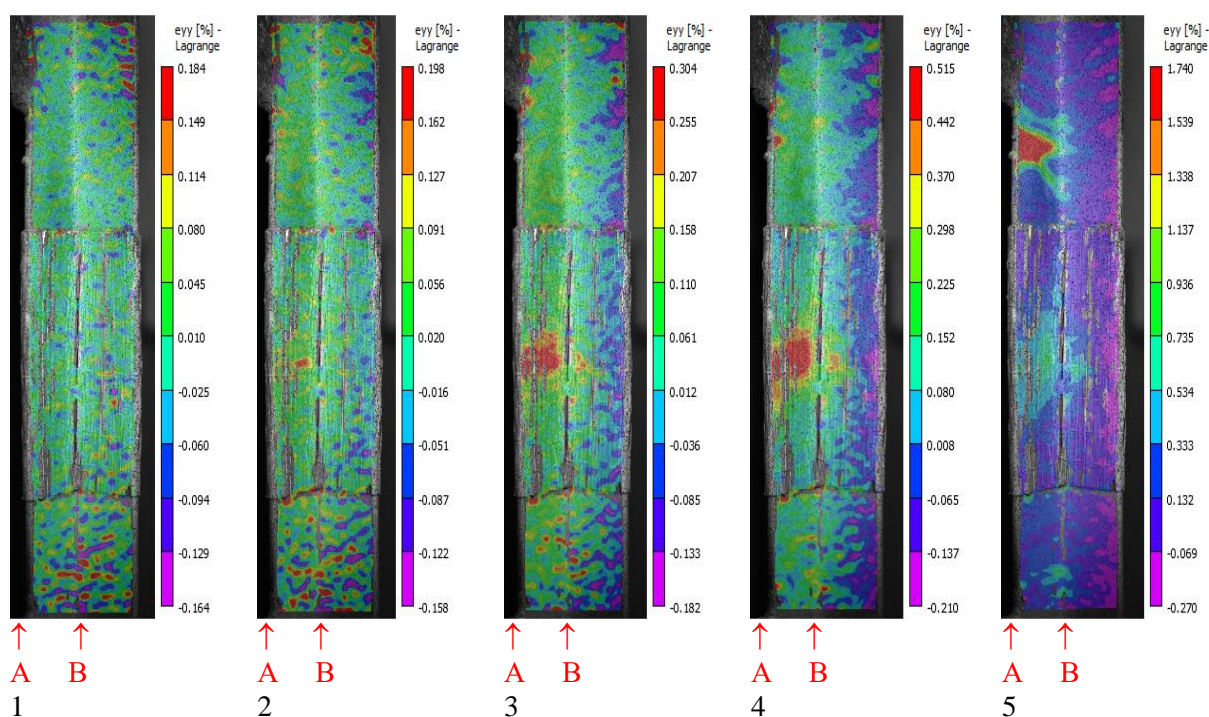
Figure 3. Patterns of vertical relative deformation of the inner surfaces of a steel angle and carbon fabric plates on the different deformation phases. A – loaded side of the angle; B – not loaded side of the angle. 1, 2, 3, 4, 5 — points in the figure 2
