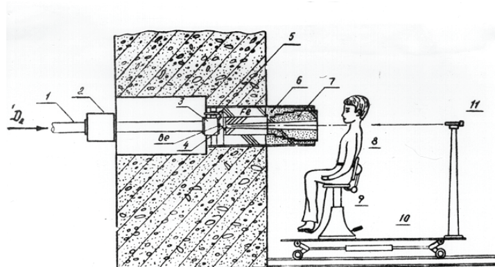
FIGURE 1. Therapeutic neutron beam scheme and the position of the patient during irradiation session. Radiation is carried out with the horizontal fixed bunch, at 110 cm distance from a target: 1, 2—ionconductor, 3—beryllium target camera, 4—beryllium target, 5—iron shielding, 6—polyethylene shielding, 7—removable plastic collimator, 8–10—parts of the treatment chair, 11—laser therapy device
