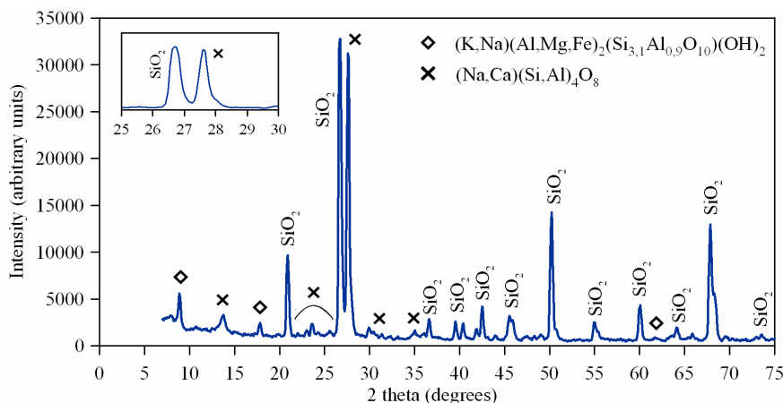
Fig. 3. XRD pattern of the fraction > 2 mm
