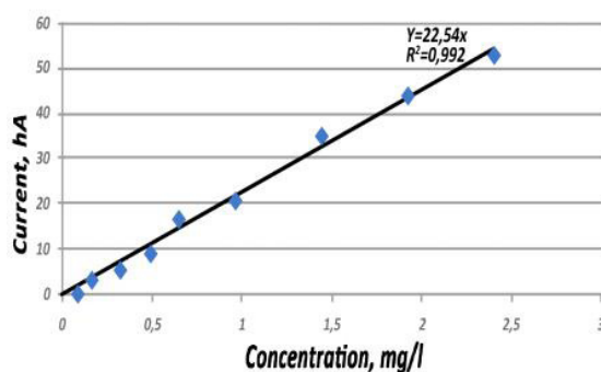
Fig. 7. Dependence of the peak current of 4-chlordehydromethyltestosterone on its concentration in phosphate electrolyte upon the concentration. ( \tau_e = 15 s; w = 20 mV/s; E_e = 0.4 V).
