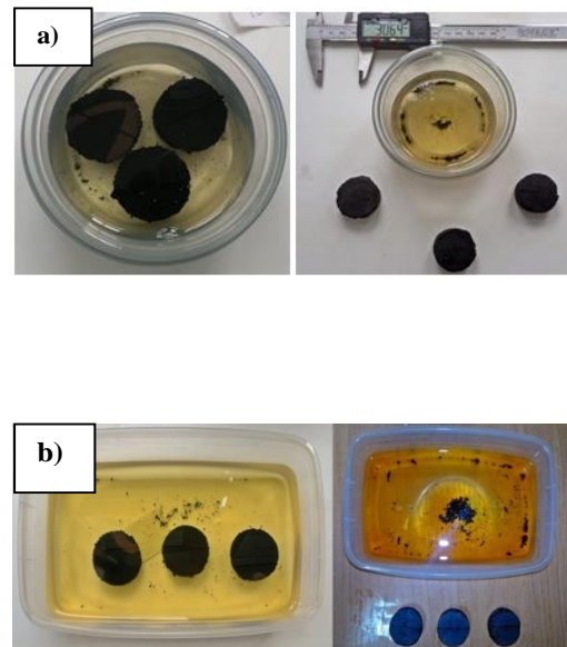
Figure 2. The samples and diesel fuel throughout 24 hours (left) and 480 hours (right), a) at 25^{\circ}\text{C} ; b) at 50^{\circ}\text{C}
