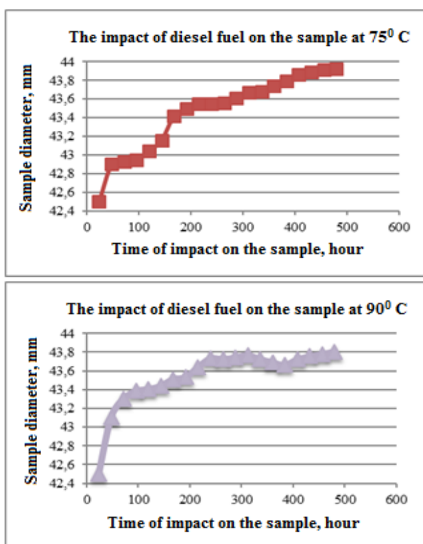
Figure 3. The impact of diesel fuel on the samples at 75 0 and 90 0 C
