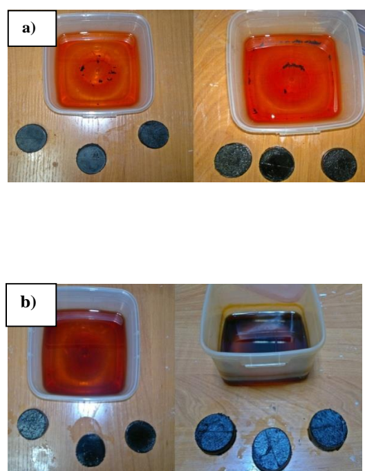
Figure 4. The samples and diesel fuel throughout 24 hours (left) and 480 hours (right), a) at 75 0 C; b) at 90 0 C
