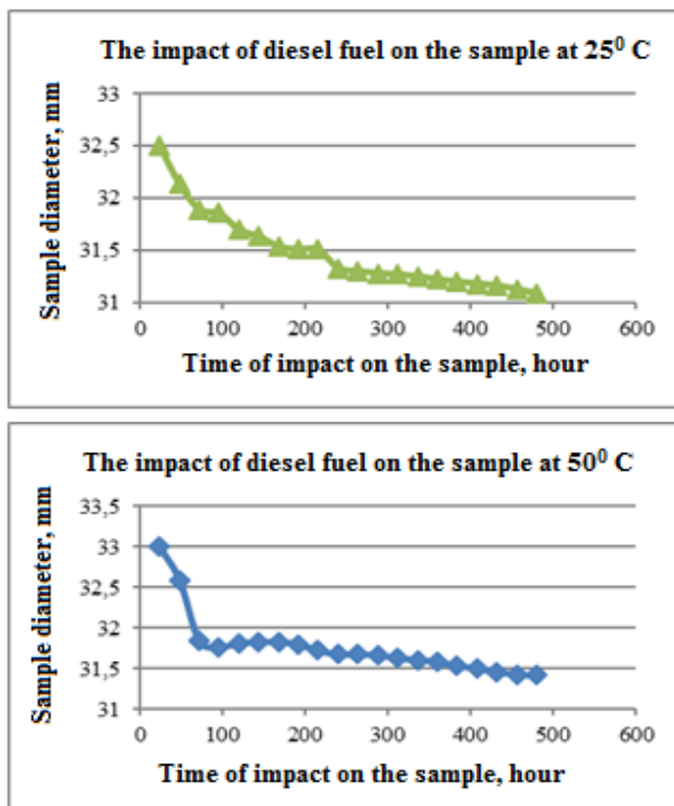
Figure 1. The impact of diesel fuel on the samples at 25^{\circ} and 50^{\circ}\text{C}
