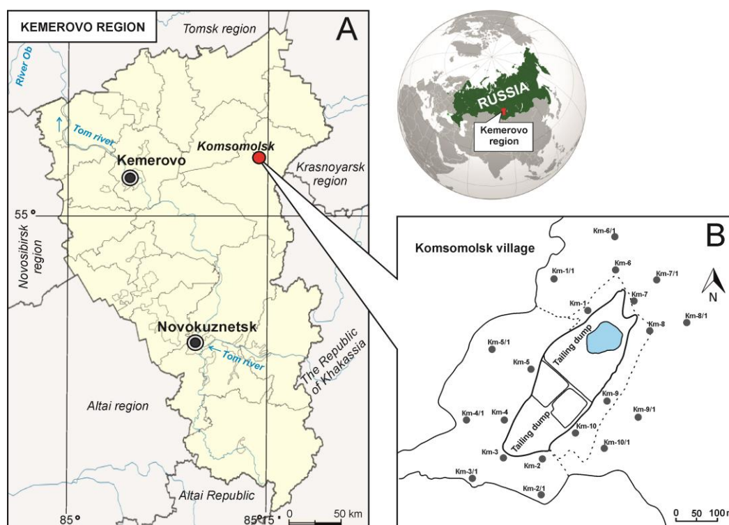
Figure 1. Map of the study area position (A), location of Komsomolsk tailing and Betula pendula leaf testing scheme (Km, ●) (B) (latitude = 55^{\circ}38'6.34'' , altitude = 88^{\circ}11'52.51'' ).
