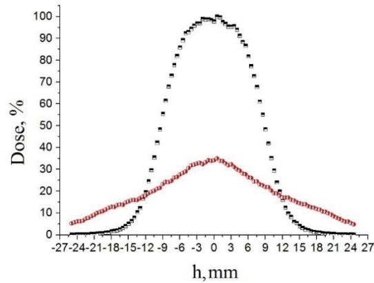
FIGURE 3. Calculated profiles of electron beams: ■ – without a filter, ◆ - with a filter
