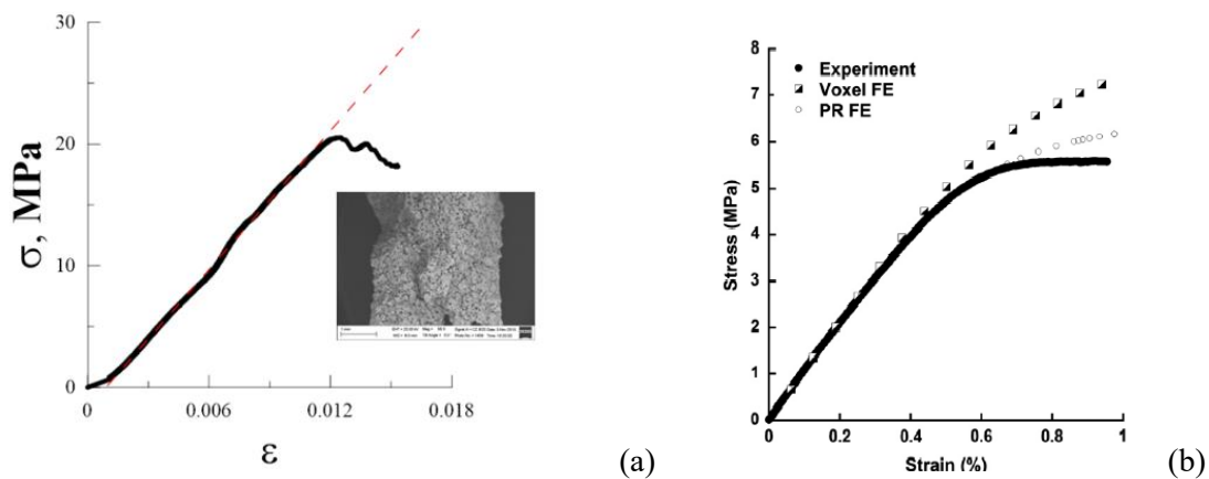
Figure 4. Stress–strain curve and macrograph of ceramic with a porosity of 40% subjected to compression (a); the stress–strain curve of human trabecular spinal bone subjected to compression (b) [10].
