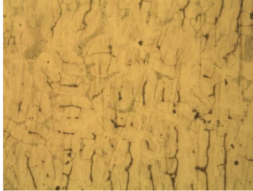
Figure 2. Structure of the faced metal (surface layer) \times 1000
