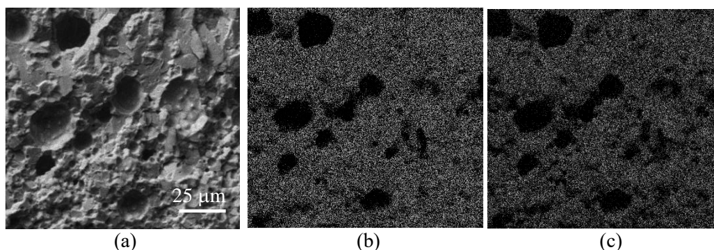
Figure 2. SEM images of fracture (a); Ti distribution (b); Nb distribution (c)
