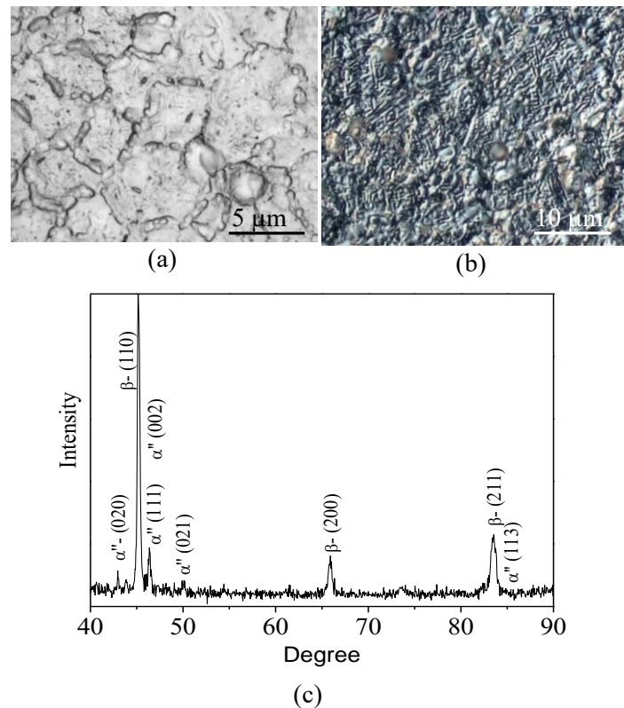
Figure 3. Optical images of the microstructure (a, b) and X-ray diffractogram fragment of the sample (c)
