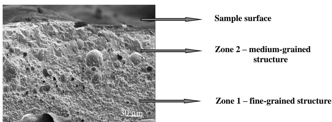
Figure 1. SEM image of fracture surface
