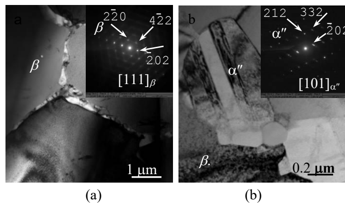
Figure 4. Light-field electron-microscopic images with corresponding microdiffractions of \beta -phase (a) and \alpha'' -phase (b)
