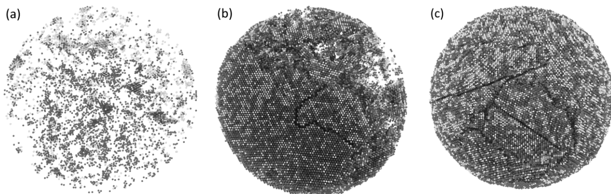
Figure 3. The final structure of the modeled sample after crystallization with different cooling rates: (a) 9.5 deg./ps, (b) 5.7 deg./ps and (c) 3.1 deg./ps.
