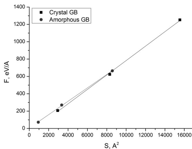
Figure 5. The dependence of adhesion strength on the area and the structure features of the molten area of two particles of Ti-Nb \beta -alloy.
