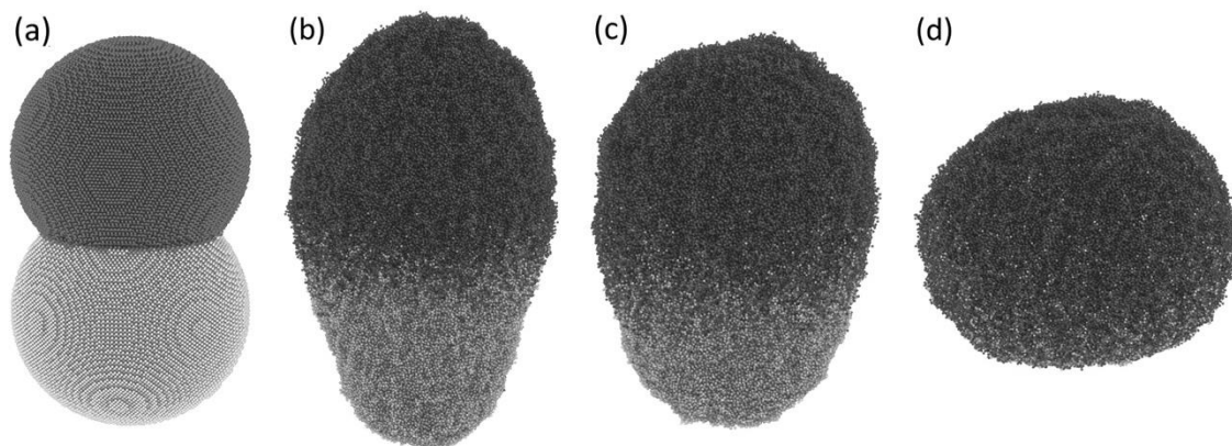
Figure 1. (a) The initial structure of the modeled particles of Ti (dark gray) and Nb (light gray) and structure corresponds to different moments of time of the high-speed heating process up to 6000K: (b) 70 ps, (c) 120 ps and (d) 220 ps.
