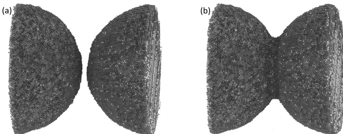
Figure 4. The structure of the modeled setup of Ti-Nb \beta -alloy at different stage: (a) before heating, (b) after heating.
