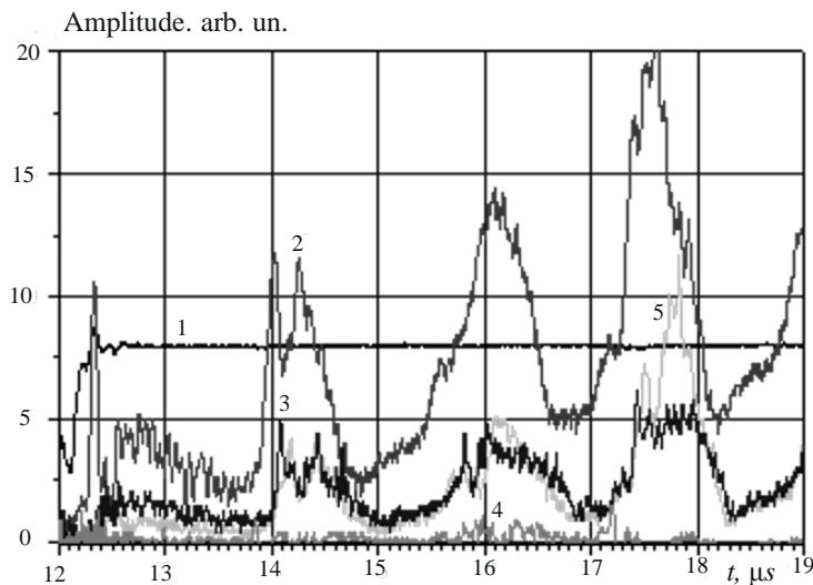
Figure 4. Oscillograms of the current and acceleration voltage. 1 is the acceleration voltage (12 kV), 2 is the target signal, 3 is the signal from the collector (displacement + 9 B), 4 is the signal from the collector (displacement +25 B), 5 is the signal from the first grid of the spectrometer.
