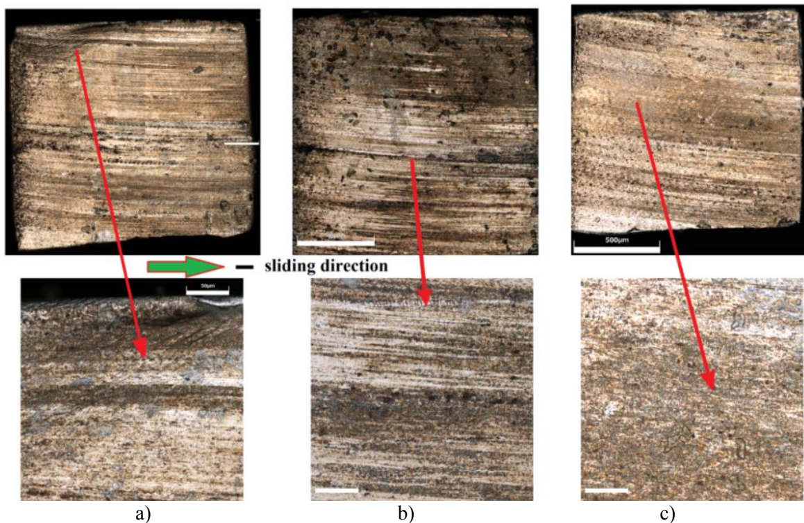
Figure 2. The friction surface of Hadfield steel single crystal: (a) - the first trial, (b) - the second trial, (c) the third trial
