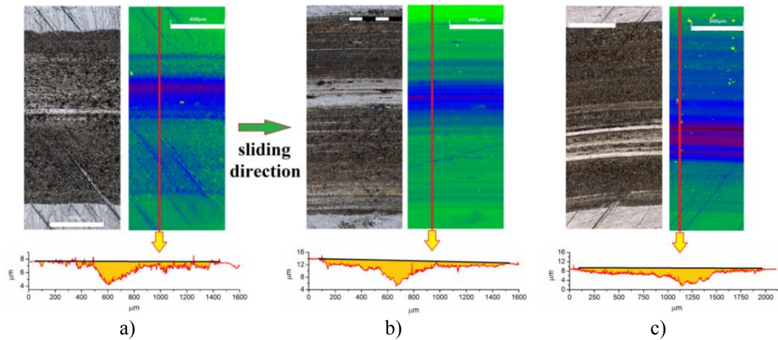
Figure 3. Images of the friction track, distribution of heights and cross section profile after the first (a), second (b) and third (c) trials.
