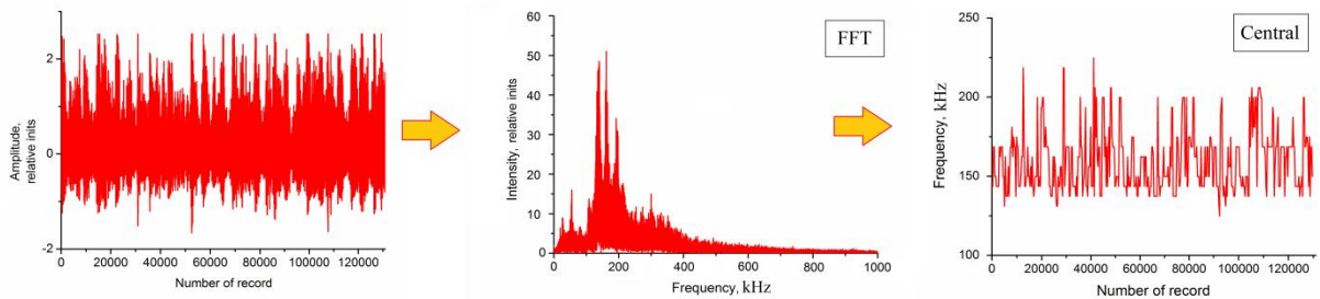
Figure 6. Typical AE signal in the run-in area in the process of Hadfield steel single crystals
