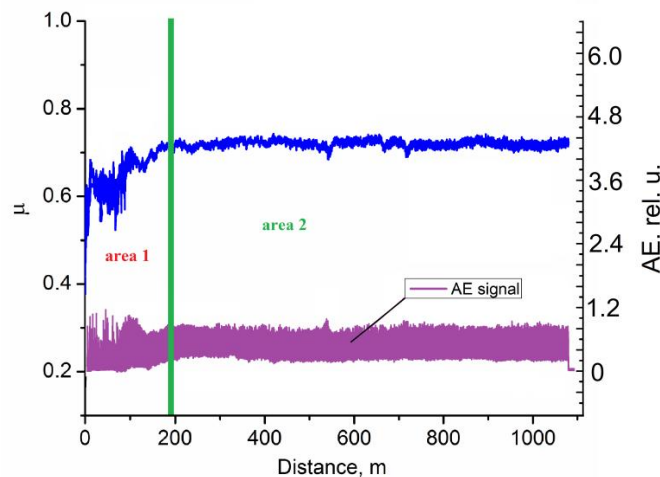
Figure 4. The change of friction factor over the three sequential trials and typical form of the waveform envelope of AE signal
