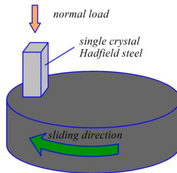
Figure 1. Scheme of «pin-on-disk» friction test
