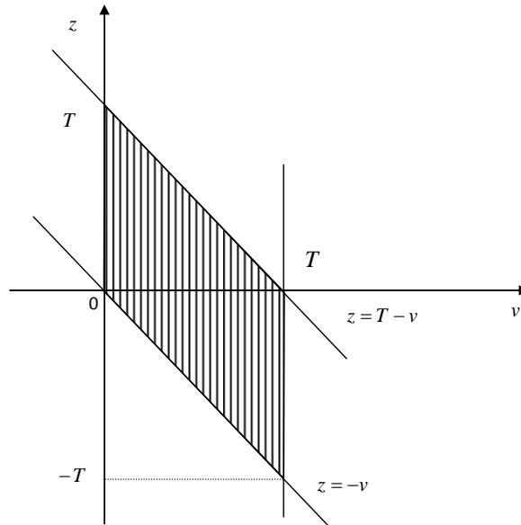
Figure 1. The range of integration.
