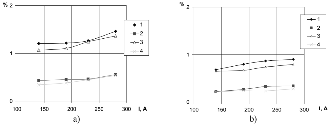
Fig. 2. The dependence of Mn and Si level in weld metal of 45 steel joint welds: a) welding with Sv-08G2S wire; b) welding with Sv-08GSMT wire. Traditional single-jet gas shielding: line 1 – Mn, line 2 – Si; Double-jet gas shielding: line 3 – Mn, line 4 – Si
