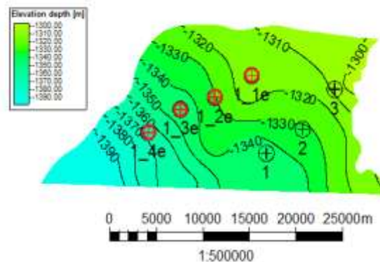
Figure 2. Structural map of block (red – modelled wells, black – real wells).
