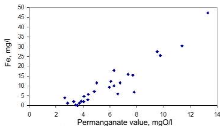
Figure 1. Iron content in the analyzed Neogene-quadernary water in dependence to permanganate value.
