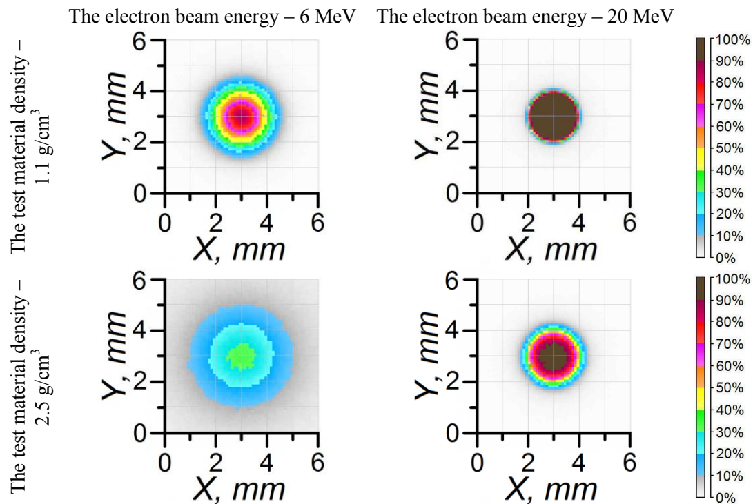
Figure 4. The electron beam shape in the transverse plane at the depth 3.67 mm in the ABS-plastic modified by zinc.
