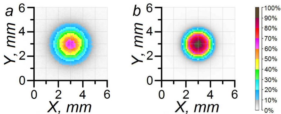
Figure 5. The electron beam shape in the transverse plane at the depth 3.67 mm in the ABS-plastic modified by a – lead and b – zinc (the test material density – 2.0 g/cm 3 ; the electron beam energy – 12 MeV).
