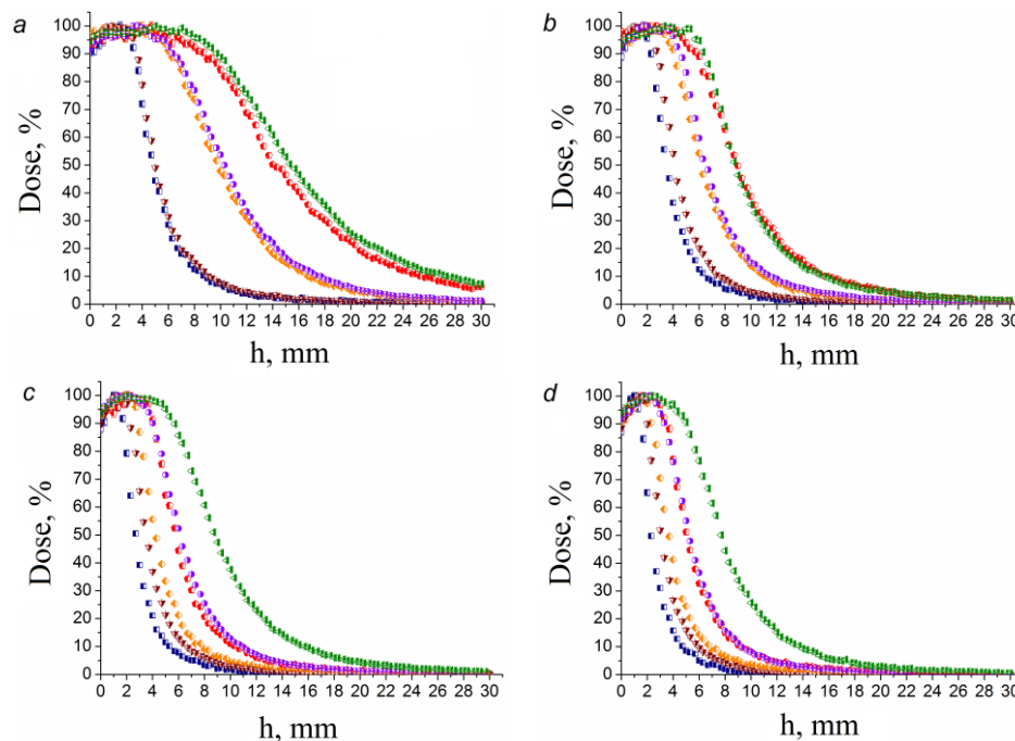
Figure 2. The electron beam depth dose distribution in the test materials with density: a – 1.1 g/cm 3 ; b – 1.5 g/cm 3 ; c – 2.0 g/cm 3 ; d – 2.5 g/cm 3 .
