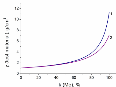
Figure 1. The dependence between the test material density and the concentration of: 1 – lead and 2 – zinc.
