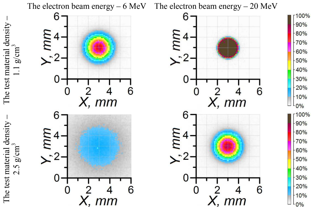
Figure 3. The electron beam shape in the transverse plane at the depth 3.67 mm in the ABS-plastic modified by lead.
